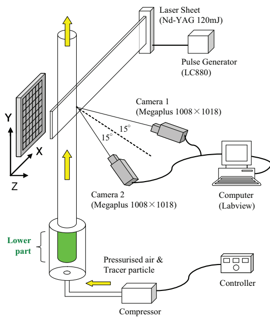
Fig. 15. Experimental setup.
